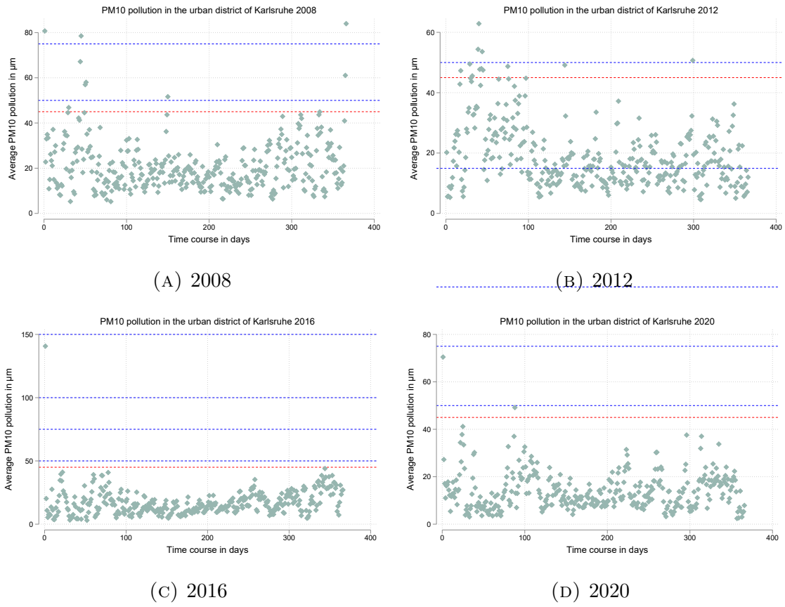
FIGURE B.5: PM 10 pollution in Karlsruhe (district 8212)
